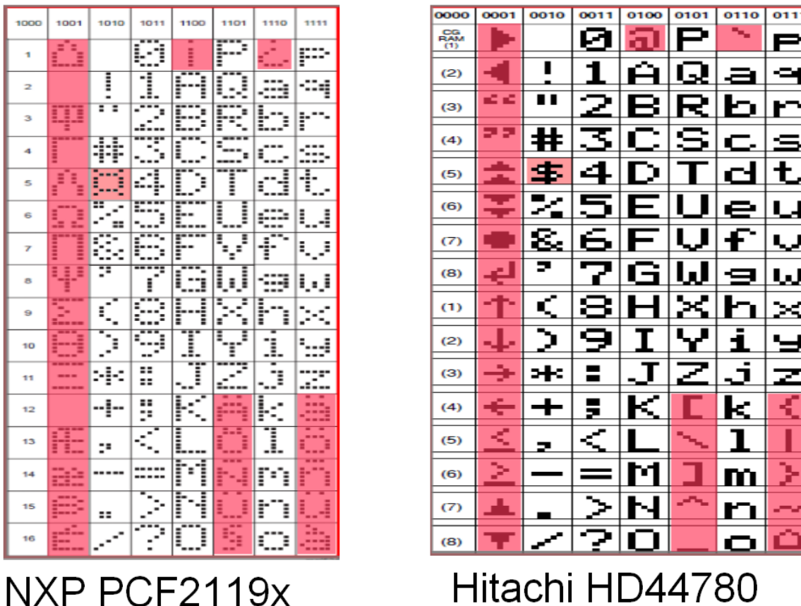
Figure 2. Character Sets for NXP PCF2119x and Hitachi HD44780 LCD Modules
