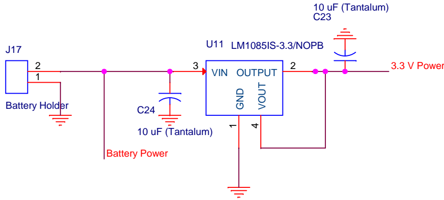
Power Supply
