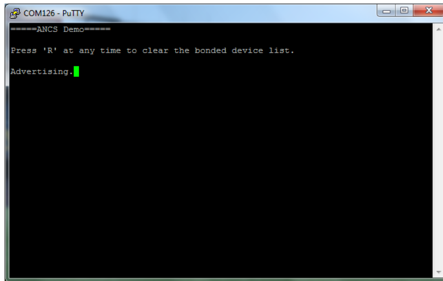
Figure 2. Terminal output
