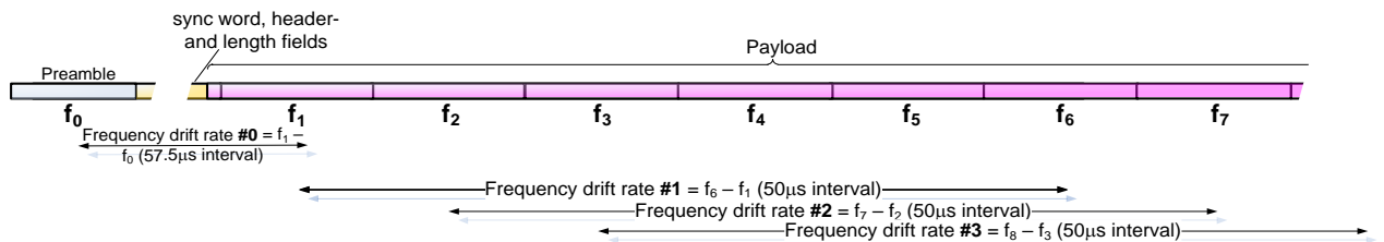
Figure 4.5: Frequency drift rate measurement principle
