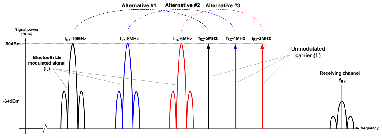
Figure 4.16: Test signal allocation alternatives in the frequency domain at 1 Ms/s. Note: figure shows only frequencies below f_0 .
