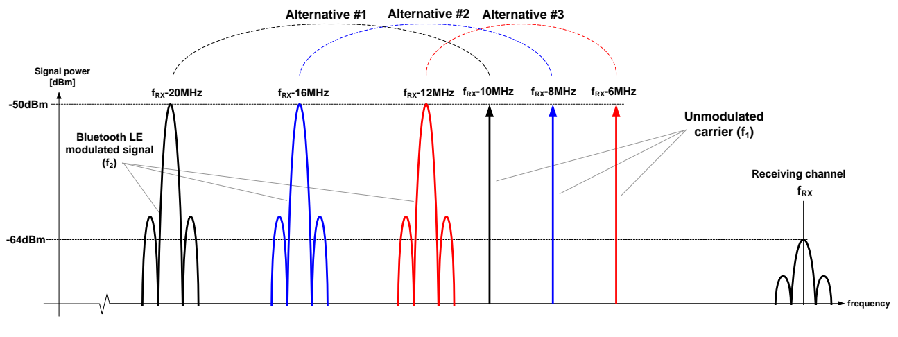
Figure 4.18: Test signal allocation alternatives in the frequency domain for 2 Ms/s. Note: figure shows only frequencies below f_0 .
