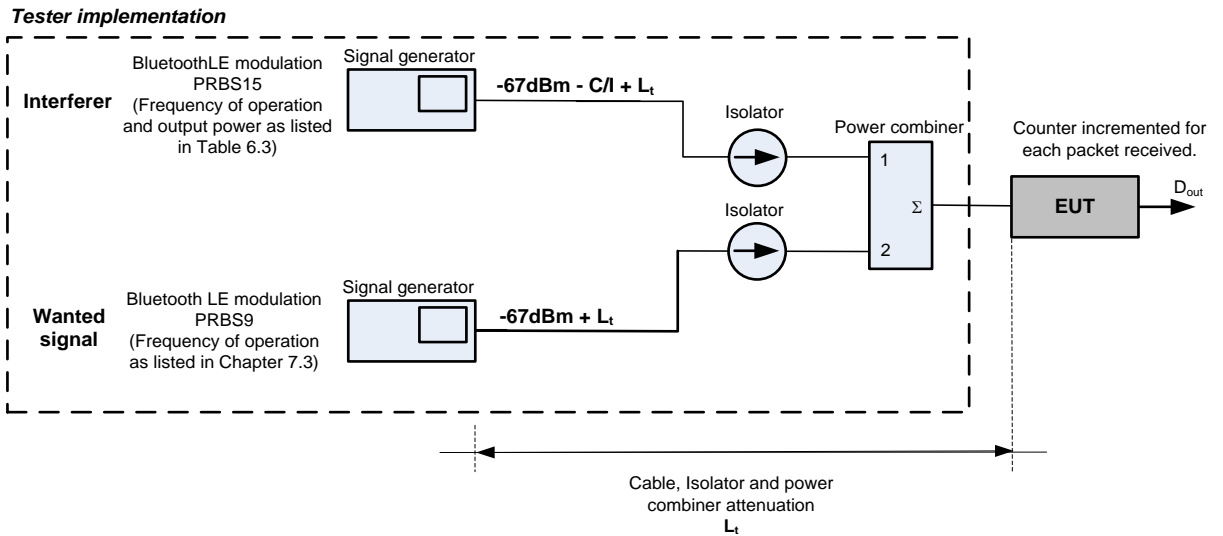
Figure 4.13: C/I- and receiver selectivity test implementation principle
