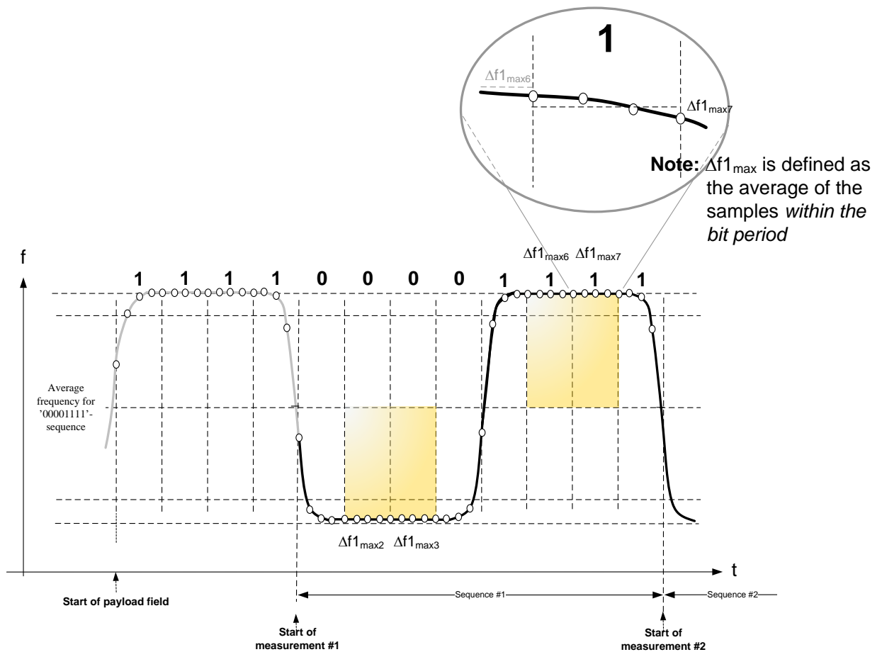
Figure 4.1: Frequency deviation measurement principle for 11110000-payload sequence
