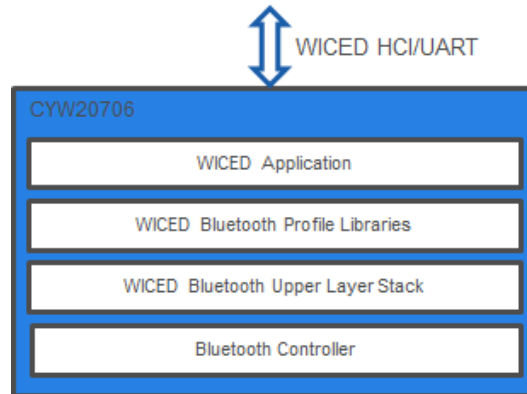
Figure 1-1. CYW20706 WICED Architecture
