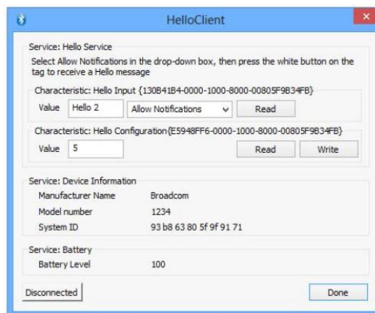
Figure 4-3. Hello Client Services Window
