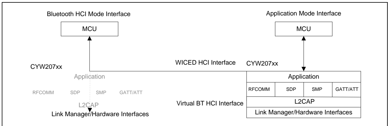
Figure 1-1. CYW207xx MCU Interfaces in the Bluetooth HCI and Application Modes
