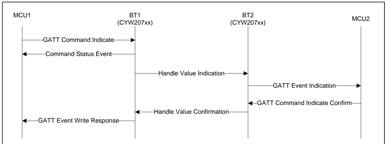
Figure 4-9. GATT Command Indicate Message Sequence
